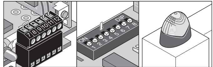
Terminals 11 + 12 Unregulated DC 24 V (max. 34 V), max. 1 A
