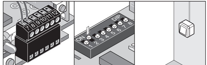
Terminals 7 + 8 Connection for button 2 only if DIP switch 2 ON
